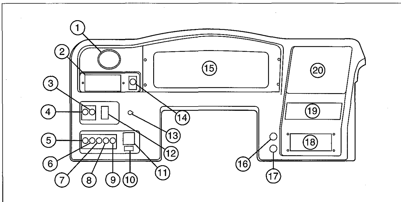
INSTRUMENT PANEL - WORKHORSE
